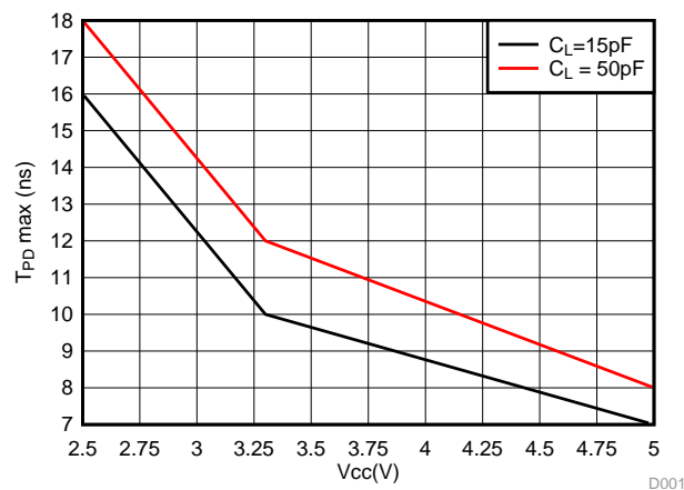
Figure 14. Maximum Propagation Delay vs V CC D001
