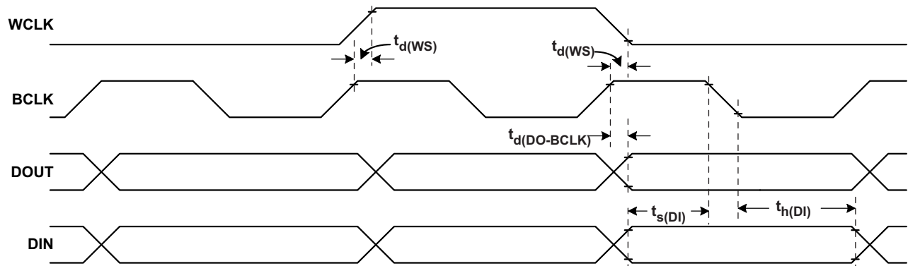
Figure 42. DSP Timing in Master Mode
