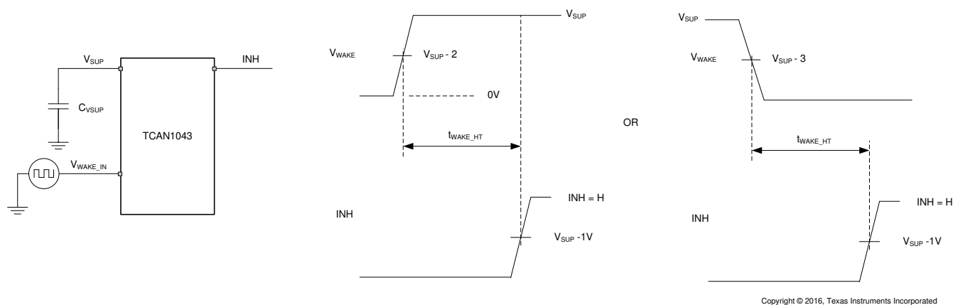
图 8-12. t_{Wake\_HT} While Monitoring INH Output
