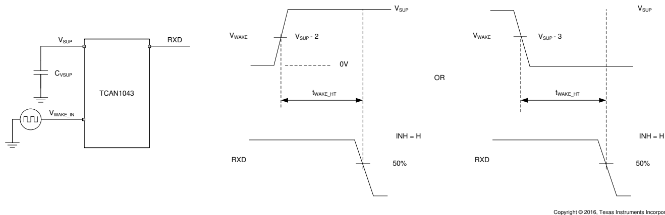
图 8-13. t_{Wake\_HT} While Monitoring RXD Output
