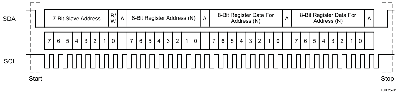
Figure 35. Typical I 2 C Sequence
