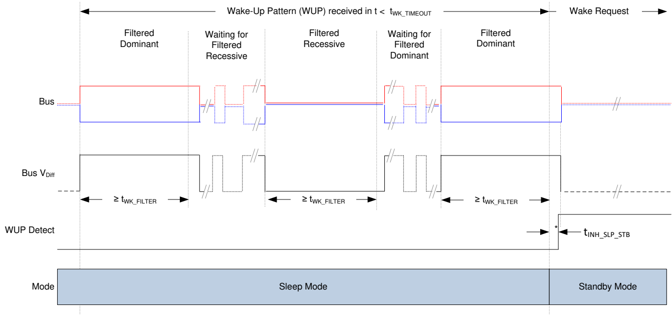
图 9-15. Wake-Up Pattern (WUP) From Sleep Mode To Standby Mode
