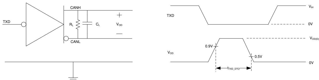
图 8-7. TXD Dominant Timeout Test Circuit and Measurement
