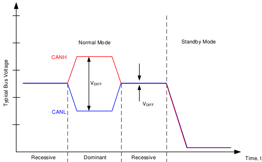
图 9-20. Bus States
