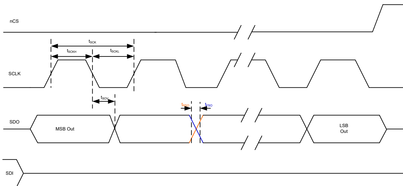
图 8-13. SPI AC Characteristic Read
