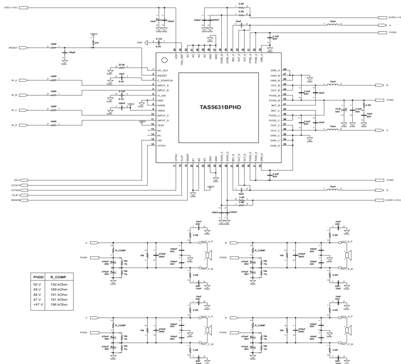
Figure 16. Typical SE Application
