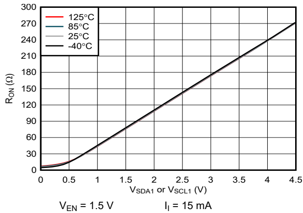
图 6-1. On-Resistance ( R_{ON} ) vs Input Voltage ( V_{SDA1} or V_{SCL1} )
