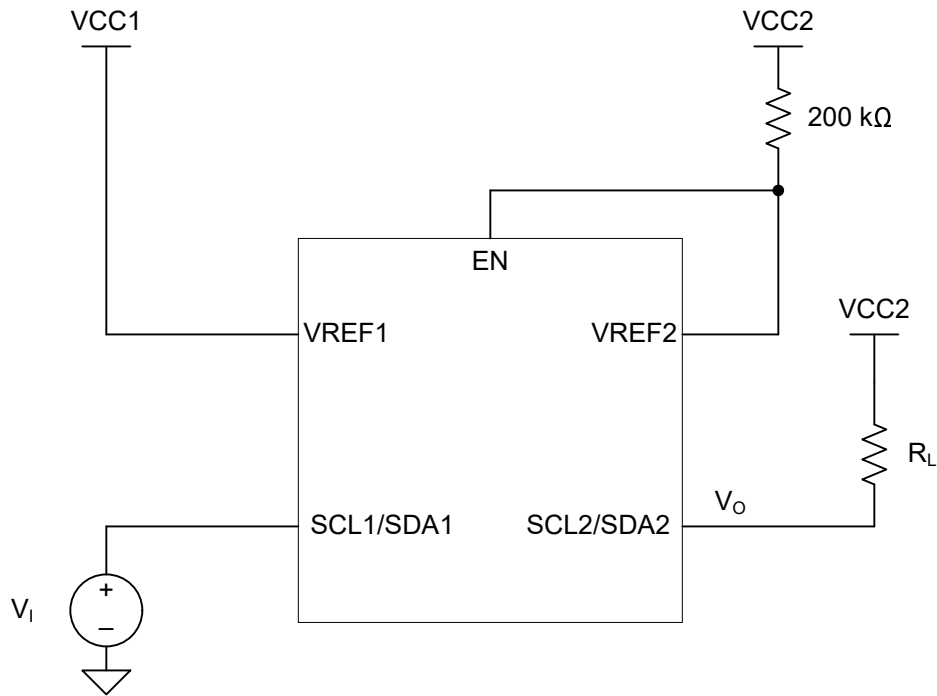
图 7-4. Application Setup for Propagation Delays Delay
