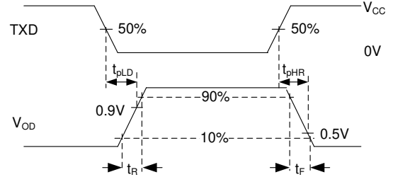
图 8-1. Driver Test Circuit and Measurement
