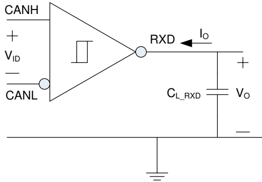
图 8-2. Receiver Test Circuit and Measurement
