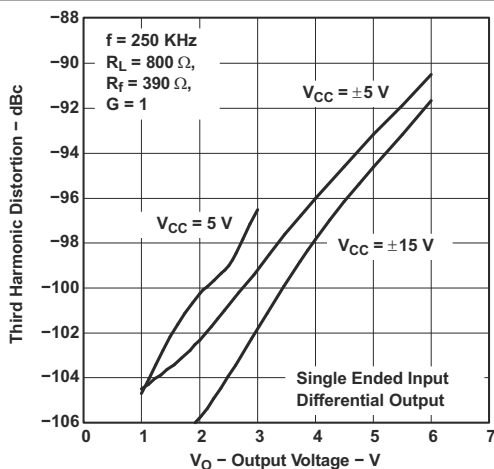
Figure 7-51. Third-Harmonic Distortion vs Output Voltage
