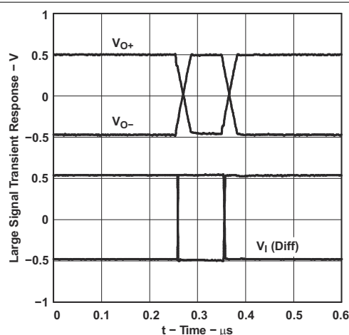
Figure 7-34. Large-Signal Transient Response (Differential In/Single Out)
