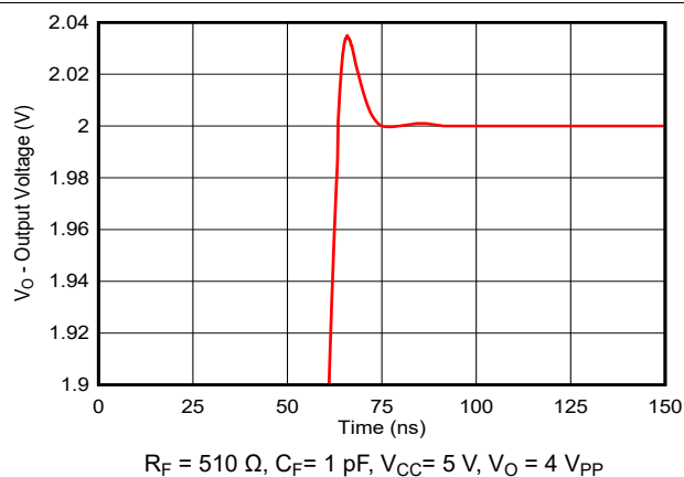
Figure 7-12. Settling Time
