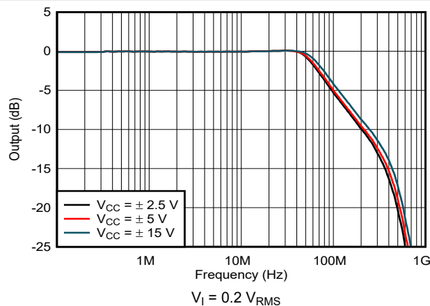
Figure 7-7. Large-Signal Frequency Response
