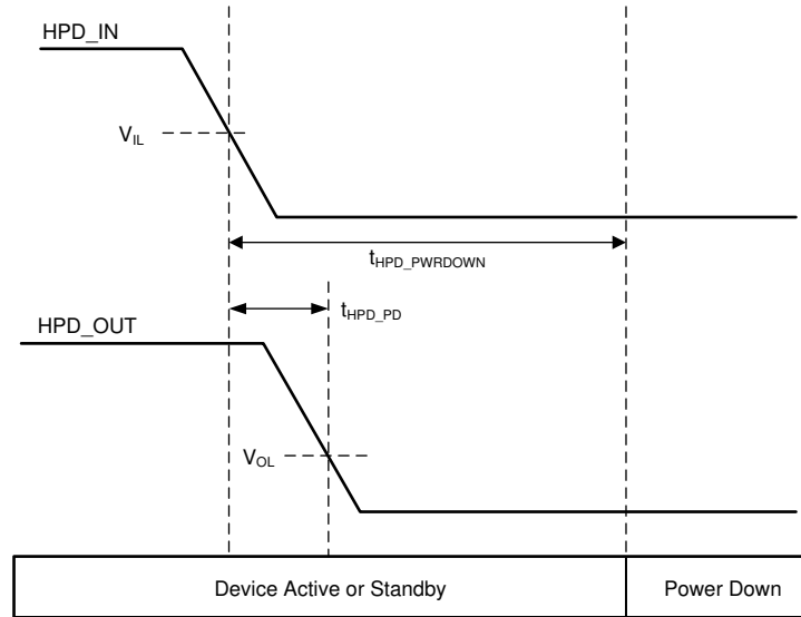
图 7-7. HPD Logic Shutdown and Propagation Timing
