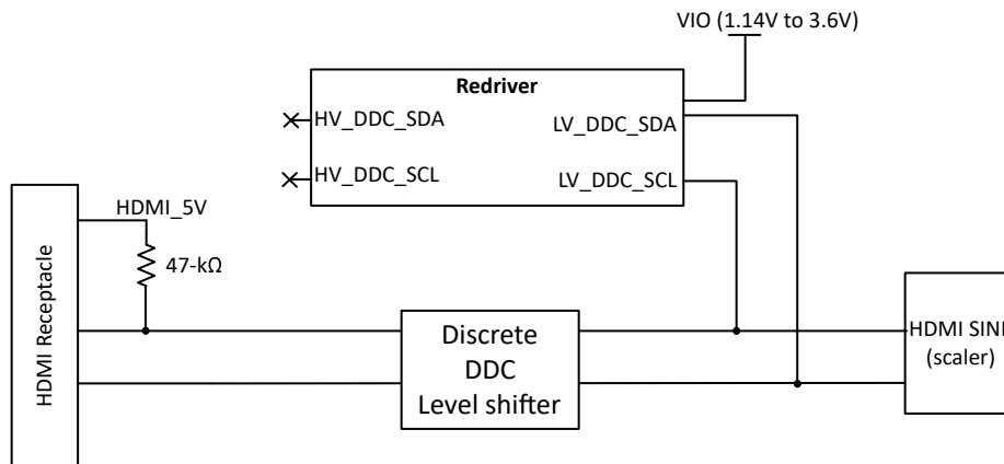
图 8-9. Sink Application: DDC Buffer Disabled and Snoop from LV DDC pins
