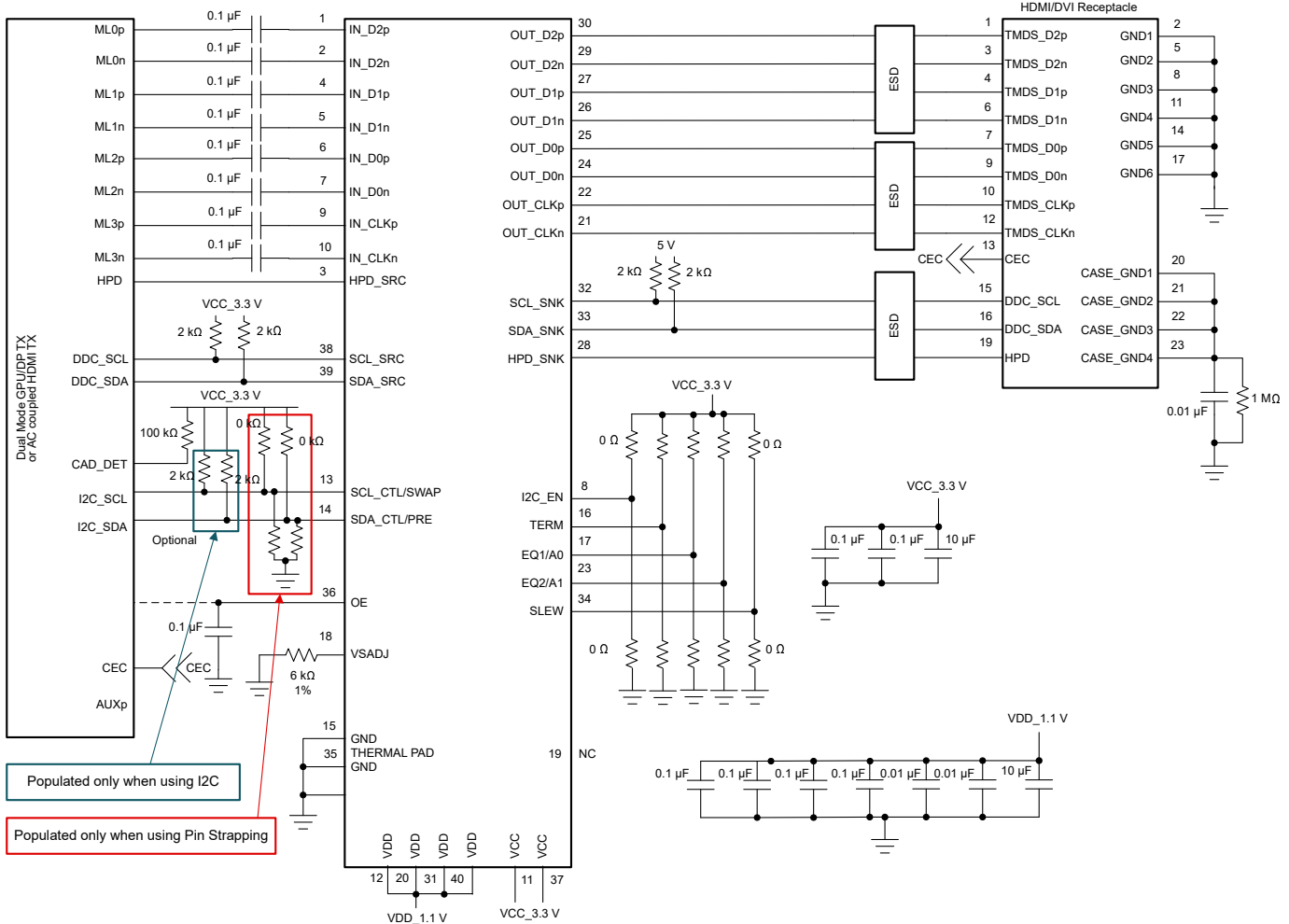
图 9-5. TDP158 Source Side Application with DDC Snoop
