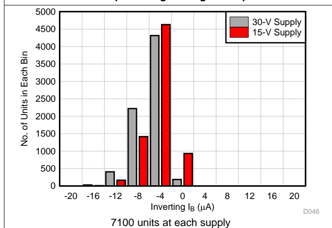
图 33. Inverting I_B Distribution
