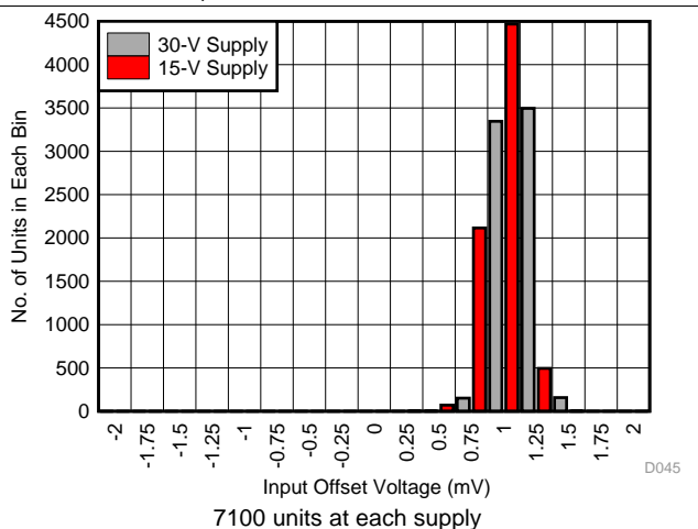
图 32. Input Offset Voltage Distribution
