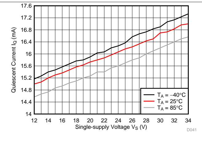
图 30. Quiescent Current vs Supply Voltage
