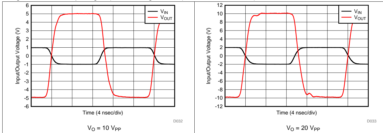
图 25. G = -5\text{ V/V} Pulse Response
