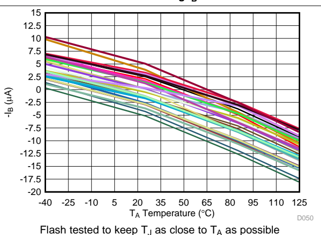
图 36. Inverting I_B Over Temperature
