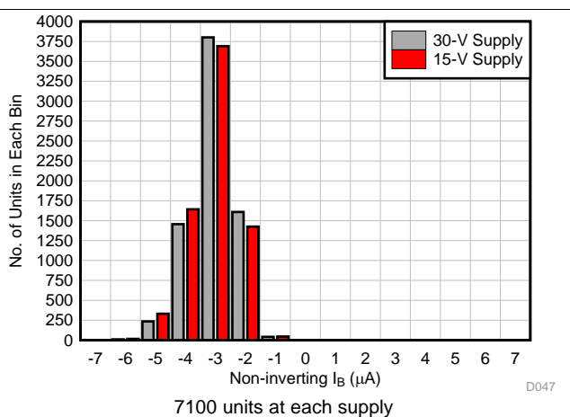
图 34. Noninverting I_B Distribution
