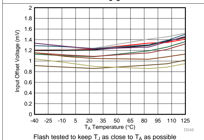
图 35. Input Offset Voltage Over Temperature
