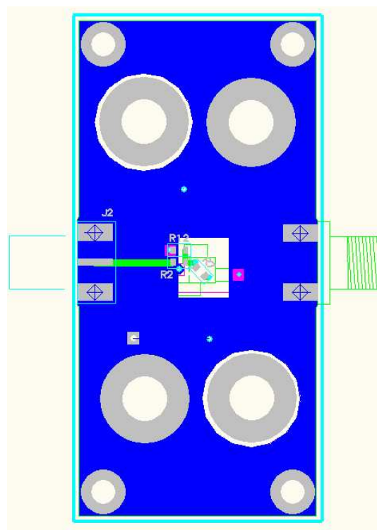
Figure 51. THS4304DBV EVM Layout Bottom and L3
