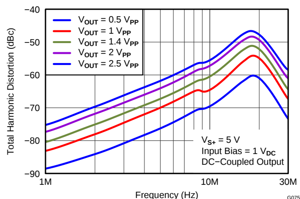
Figure 87. HD THD vs FREQUENCY
