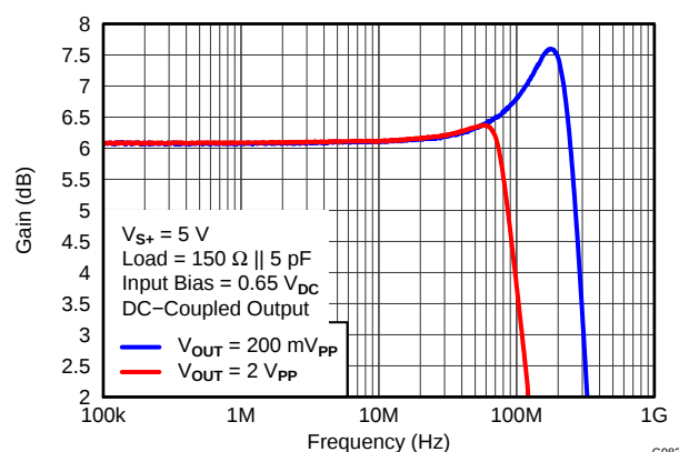
Figure 97. HD BYPASS LARGE-SIGNAL GAIN vs FREQUENCY
