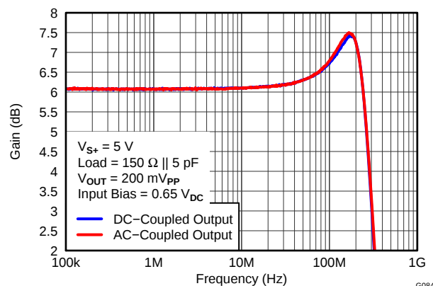
Figure 99. HD BYPASS SMALL-SIGNAL GAIN vs FREQUENCY
