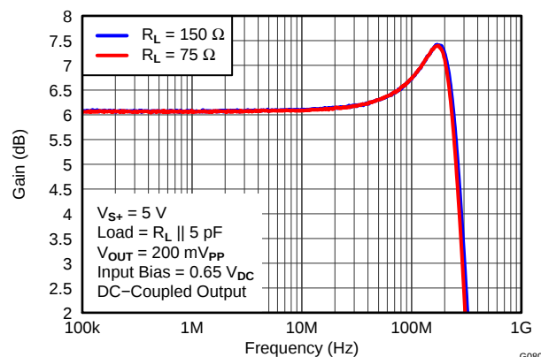
Figure 95. HD BYPASS SMALL-SIGNAL GAIN vs FREQUENCY
