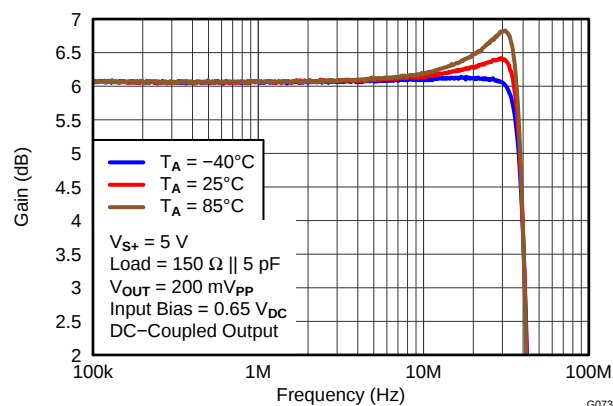
Figure 85. HD SMALL-SIGNAL GAIN vs FREQUENCY
