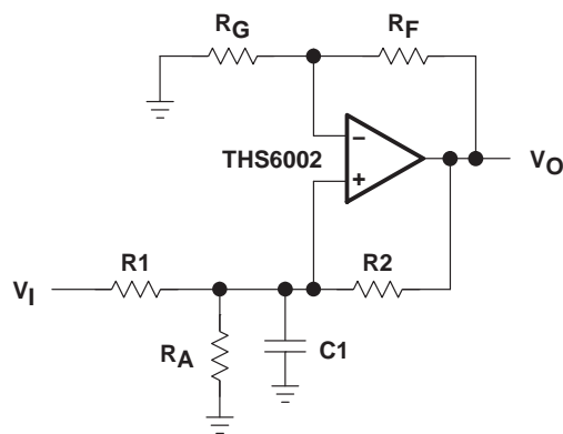
Figure 64. Non-Inverting CFB Integrator
