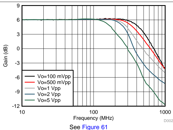
Figure 2. Frequency Response vs Vpp
