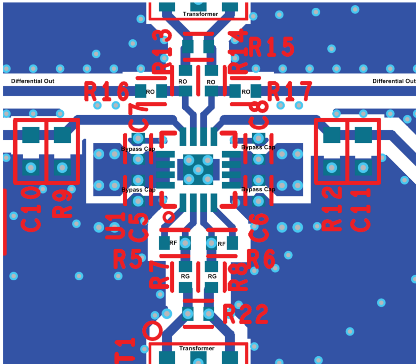
Figure 82. Layout Example
