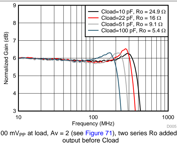
Figure 5. Small-Signal Frequency Response vs Load
