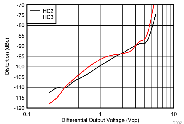
Figure 32. Harmonic Distortion vs Output Swing
