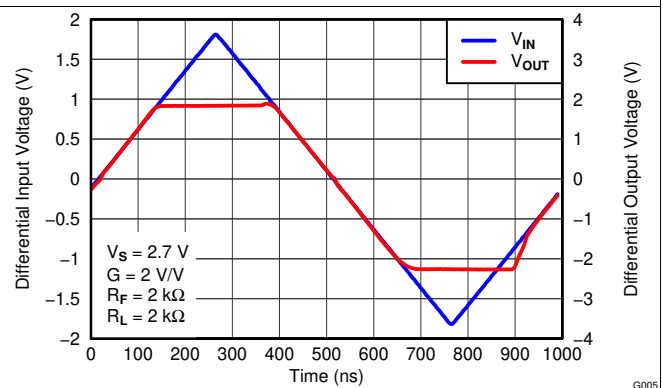
Figure 7. Overdrive Recovery
