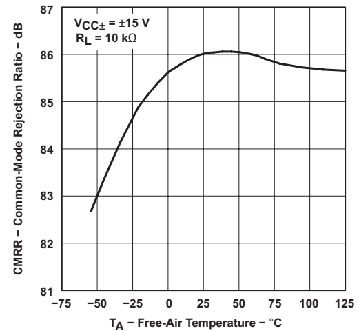
Figure 10. All Except TL061 Common-Mode Rejection Ratio vs Free-Air Temperature
