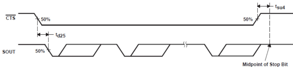
Figure 6-13. \overline{\text{CTS}} and SOUT Autoflow Control Timing (Start and Stop) Waveforms
