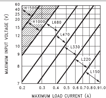
Figure 14. TL2575-50
