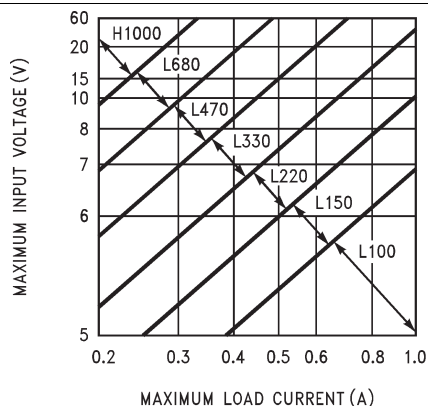
Figure 13. TL2575-33
