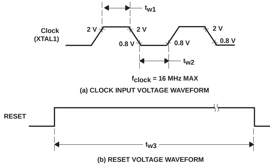
Figure 1. Clock Input and RESET Voltage Waveforms
