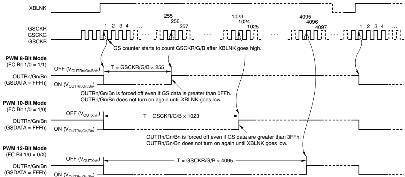
Figure 43. PWM Operation 2
