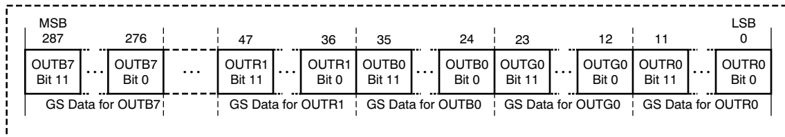
Figure 46. Grayscale Data-Latch Configuration
