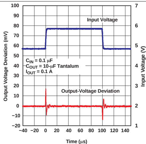
Figure 8. TLV1117-33 Line Transient Response
