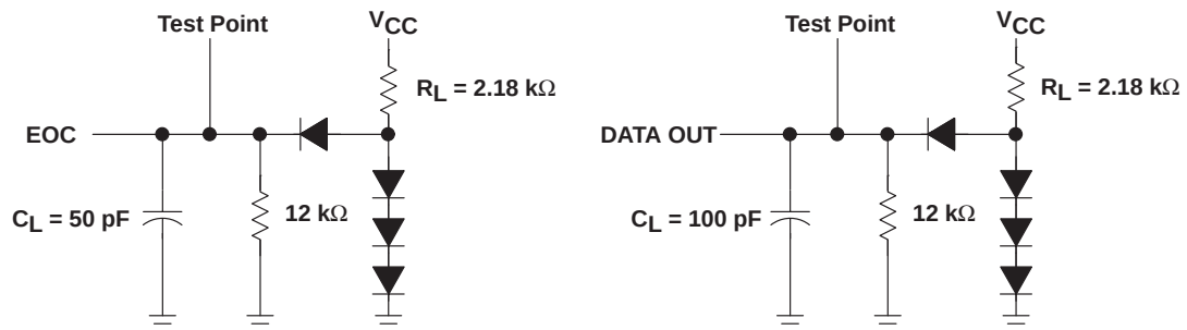
Figure 7. Load Circuits
