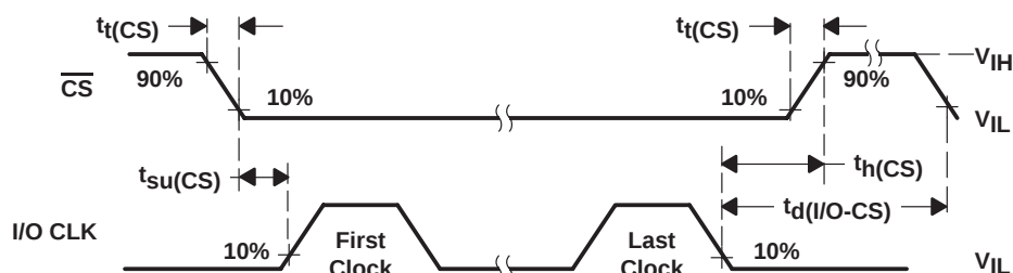
Figure 10. \overline{CS} and I/O CLK Voltage Waveforms
