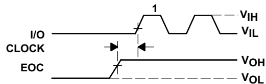
Figure 38. I/O CLOCK and DATA OUT Voltage
