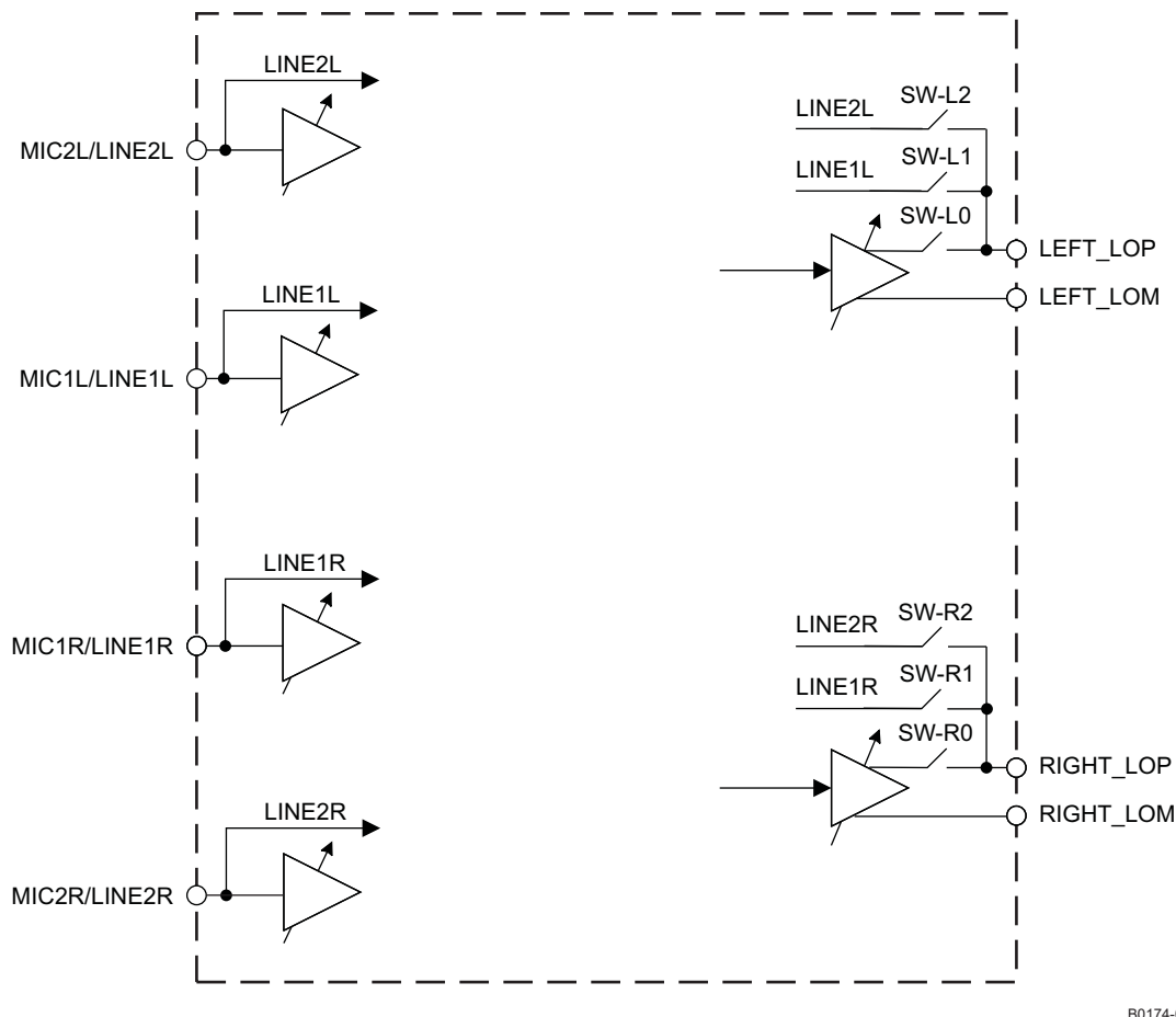
Figure 28. Passive Analog Bypass Mode Configuration
