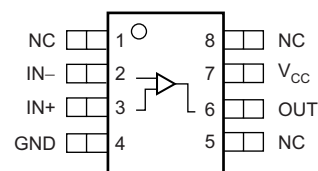
TLV3701 D or P Package 8-Pin SOIC or PDIP Top View
