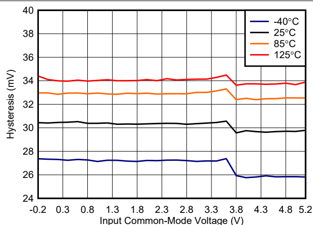
图 6-18. TLV3603 Hysteresis vs. Common-Mode, 5 V
