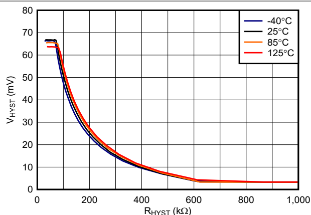
图 6-20. TLV3603 Hysteresis vs. Resistance, 3.3 V
