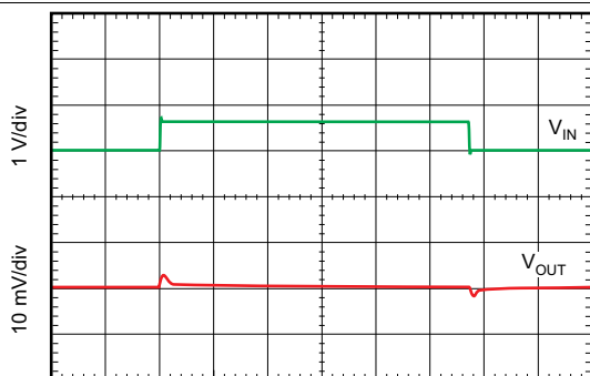
Figure 49. Line Transient Response
