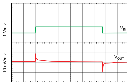
Figure 50. Line Transient Response
