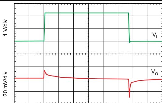
Figure 51. Line Transient Response
