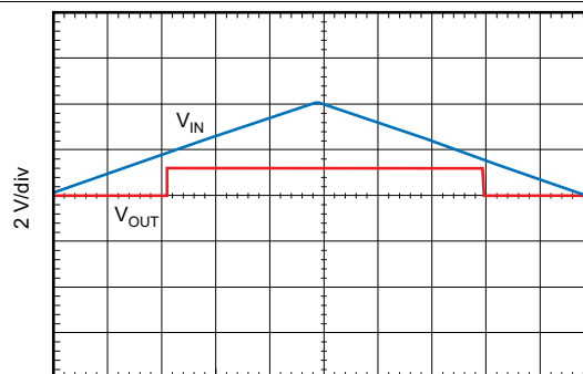
Figure 52. Line Transient Response
