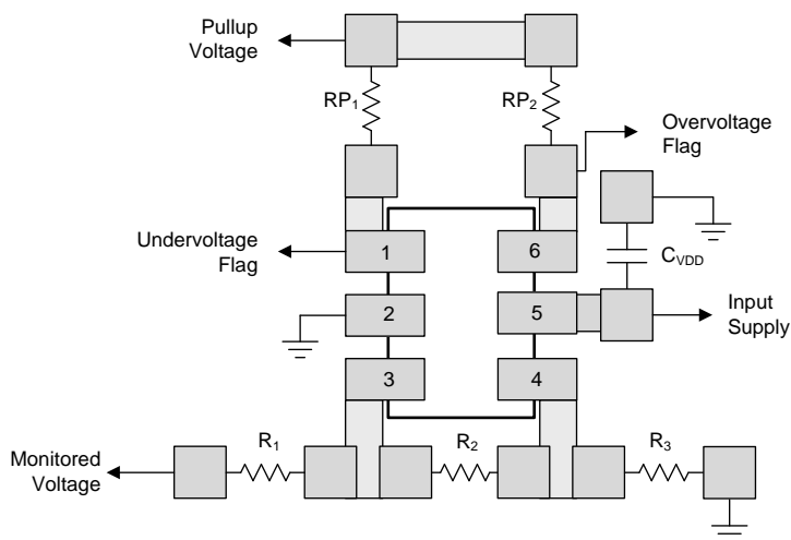
Figure 27. Recommended Layout
