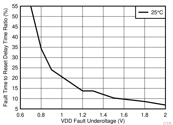
Figure 8-3. C_{CT} Discharge Time During Fault Condition ( V_{IT-} = 2.1 V, C_{CT} = 1 \mu F)
