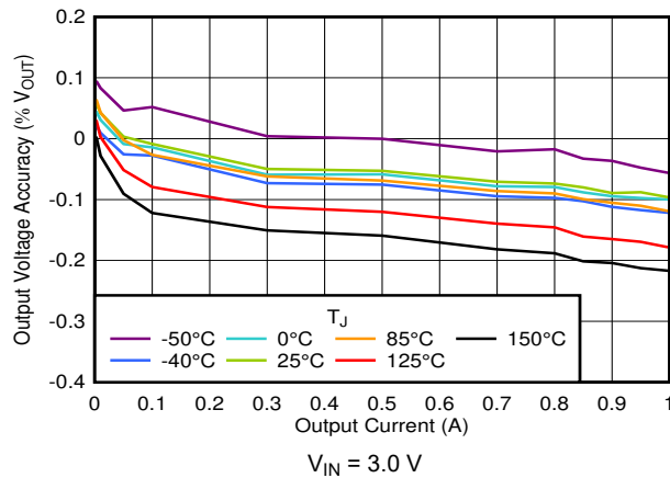
图 7-1. V_{OUT} Accuracy vs I_{OUT}
