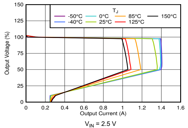
图 7-20. Foldback Current Limit vs Temperature
