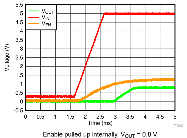
图 7-22. Startup With V_{EN} Floating
