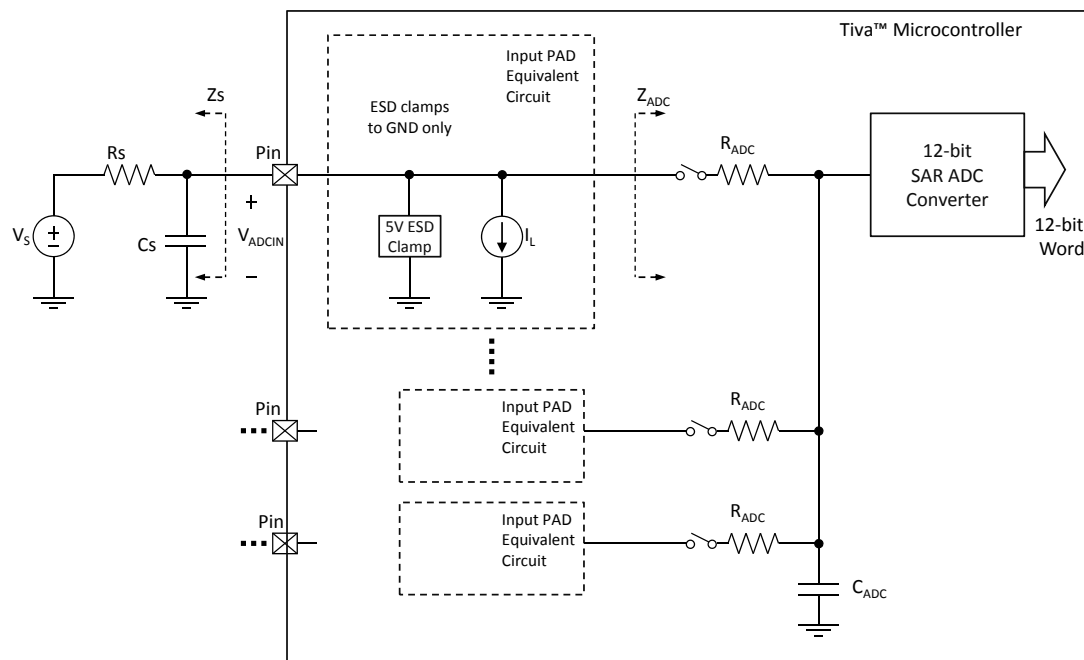
图 23-18. ADC Input Equivalency Diagram
