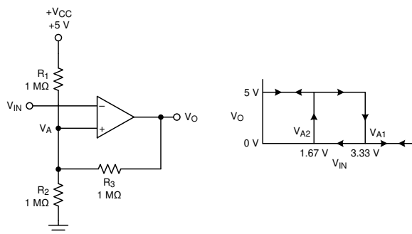
Figure 8-3. TLV903x-Q1 in an Inverting Configuration With Hysteresis
