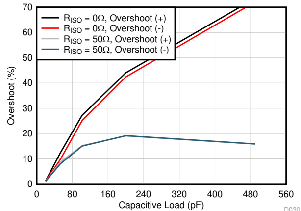
Figure 6-32. Small-Signal Overshoot vs Capacitive Load
