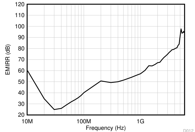
Figure 6-40. EMIRR (Electromagnetic Interference Rejection Ratio) vs Frequency
