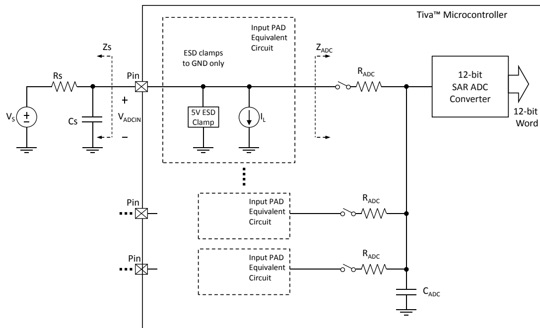
图 22-17. ADC Input Equivalency Diagram
