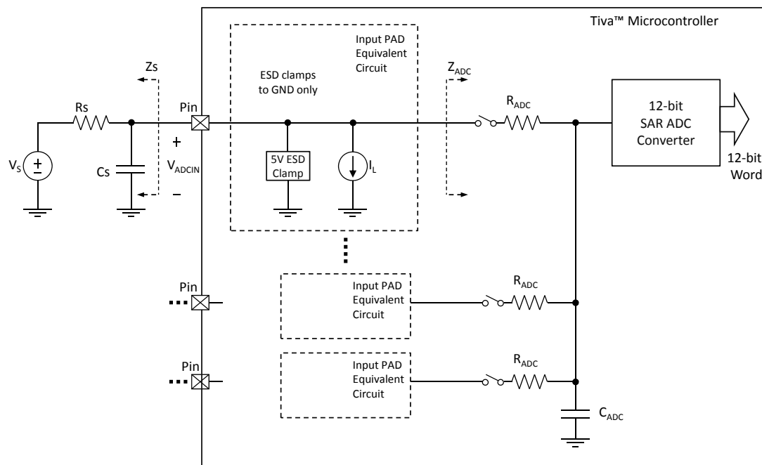
图 20-17. ADC Input Equivalency Diagram
