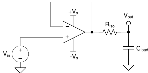
Figure 7-7. Extending Capacitive Load Drive With the TLV9161
