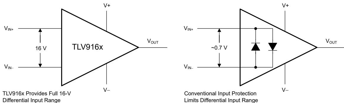
Figure 7-1. TLV916x Input Protection Does Not Limit Differential Input Capability
