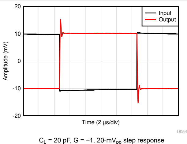
Figure 6-35. Small-Signal Step Response
