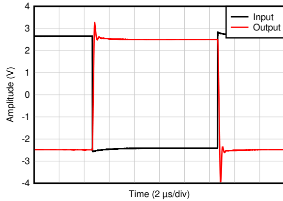
C_L = 20\text{ pF} , G = -1 , 5\text{-V}_{pp} step response Figure 6-37. Large-Signal Step Response
