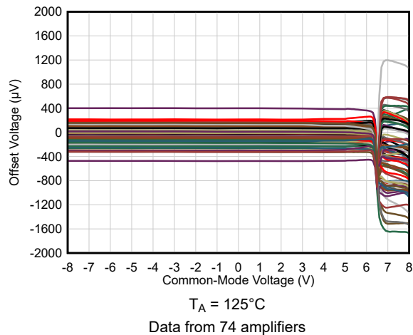
Figure 6-7. Offset Voltage vs Common-Mode Voltage
