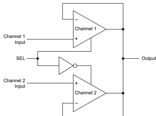
Figure 8-3. Precision Reference Buffer
