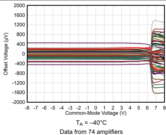
Figure 6-9. Offset Voltage vs Common-Mode Voltage
