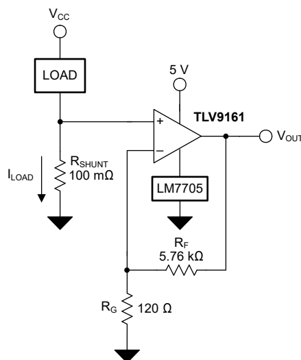
Figure 8-1. TLV9161 in a Low-Side, Current-Sensing Application
