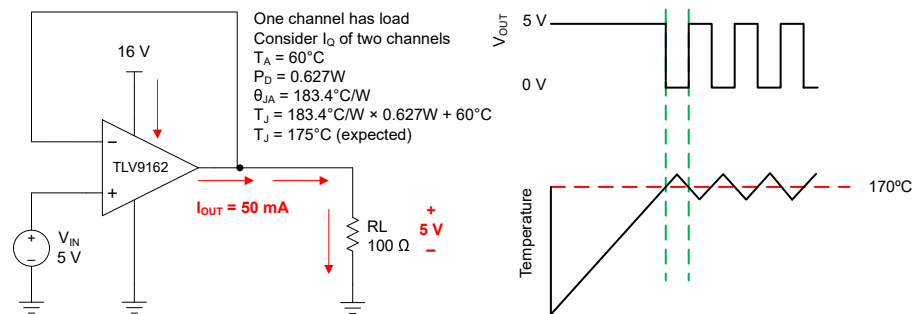
Figure 7-4. Thermal Protection
