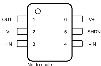
Figure 5-3. TLV9161S DBV Package 6-Pin SOT-23 (Top View)
