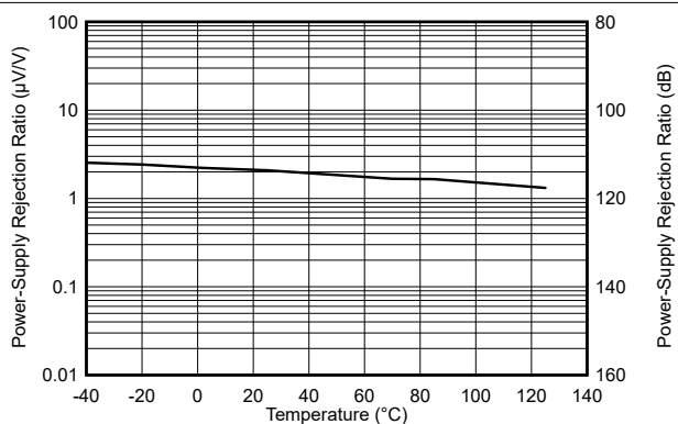
Figure 6-24. PSRR vs Temperature
