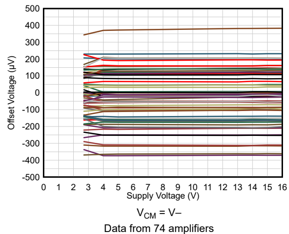
Figure 6-11. Offset Voltage vs Power Supply
