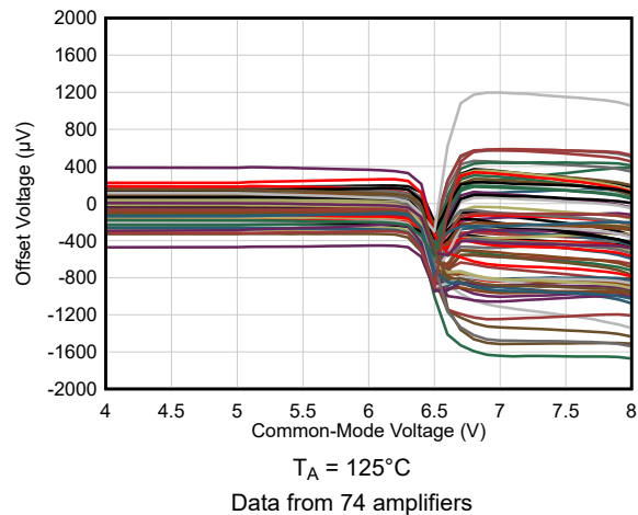
Figure 6-8. Offset Voltage vs Common-Mode Voltage (Transition Region)
