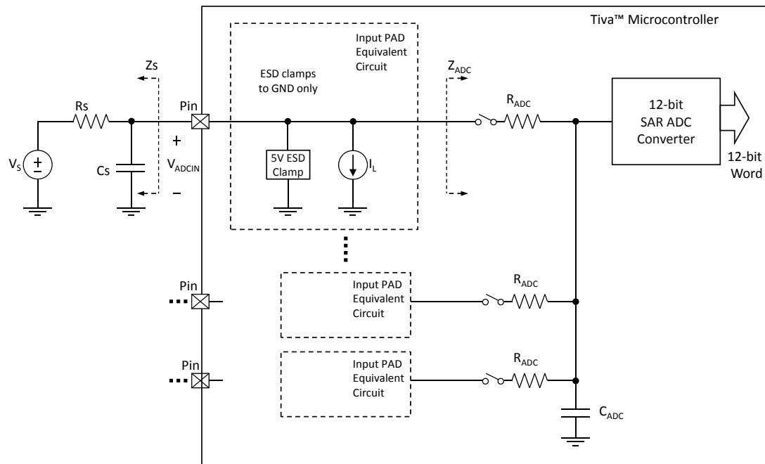
图 22-18. ADC Input Equivalency Diagram
