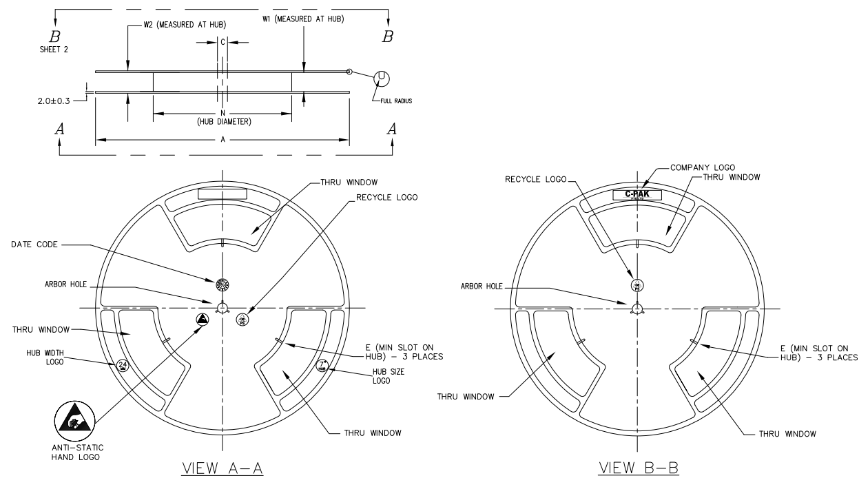
DIMENSIONS (MM)
