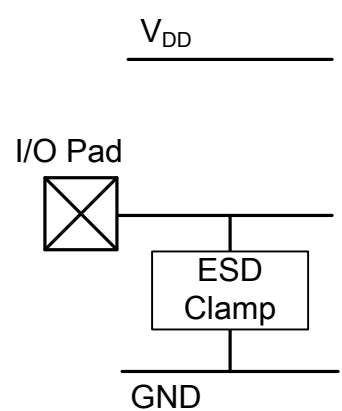
图 21-15. ESD Protection on Fail-Safe Pins
