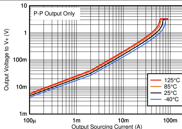
图 6-10. Output Sourcing Current vs. Output Voltage, 3.3V
