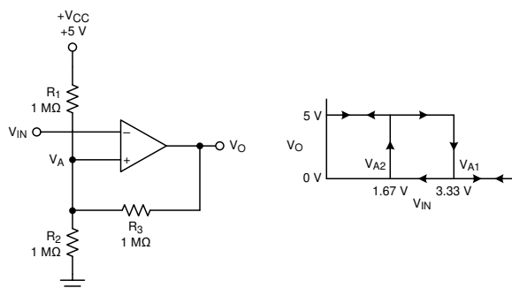
图 8-3. TLV903x-Q1 in an Inverting Configuration With Hysteresis
