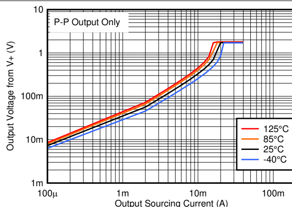
图 6-8. Output Sourcing Current vs. Output Voltage, 1.8V
