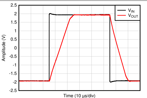
图 7-33. Overload Recovery
