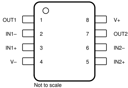
图 6-6. TLV9042 D, DDF, DGK, and PW Package 8-Pin SOIC, SOT-23 8, VSSOP, and TSSOP Top View
