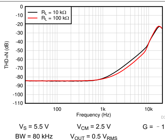
图 7-24. THD + N vs Frequency
