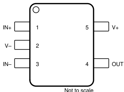
图 6-3. TLV9041 DCK Package 5-Pin SC70 Top View
