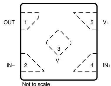
图 6-4. TLV9041 DPW Package 5-Pin X2SON Top View
