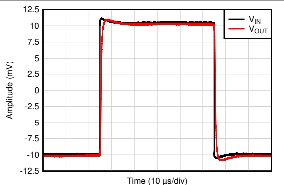
图 7-32. No Phase Reversal
