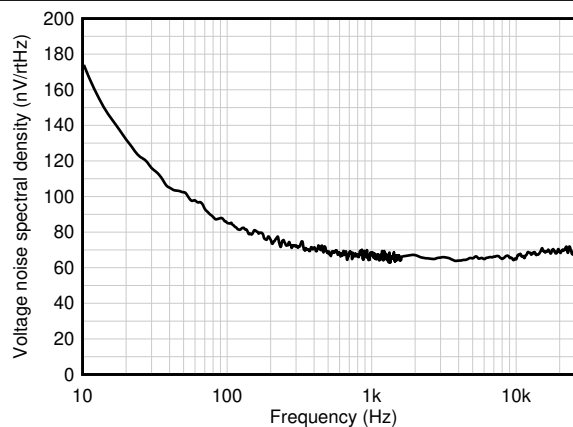
图 7-22. Input Voltage Noise Spectral Density
