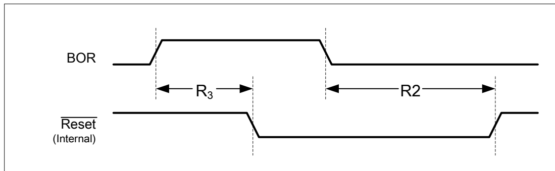
图 20-10. Brown-Out Reset Timing
