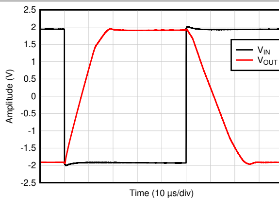
图 7-38. Large-Signal Step Response
