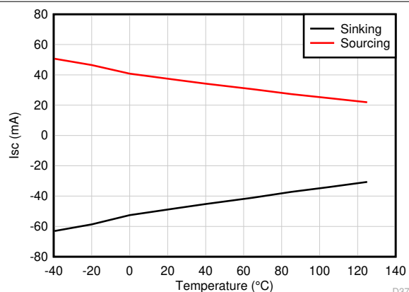
图 7-40. Short-Circuit Current vs Temperature
