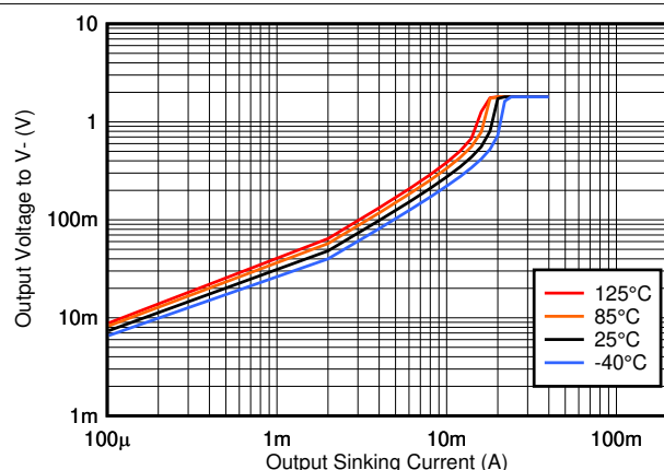
图 6-7. Output Sinking Current vs. Output Voltage, 1.8V
