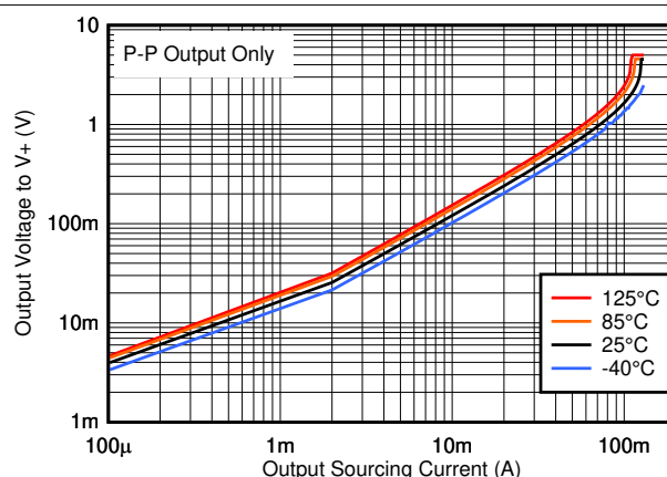
图 6-12. Output Sourcing Current vs. Output Voltage, 5V
