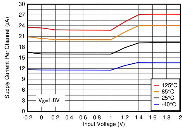
图 6-3. Supply Current vs. Input Voltage, 1.8V
