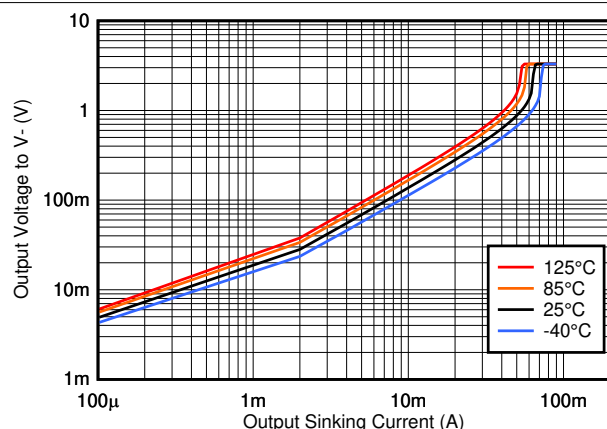
图 6-9. Output Sinking Current vs. Output Voltage, 3.3V
