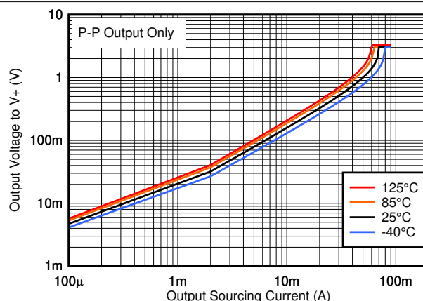
图 6-10. Output Sourcing Current vs. Output Voltage, 3.3V
