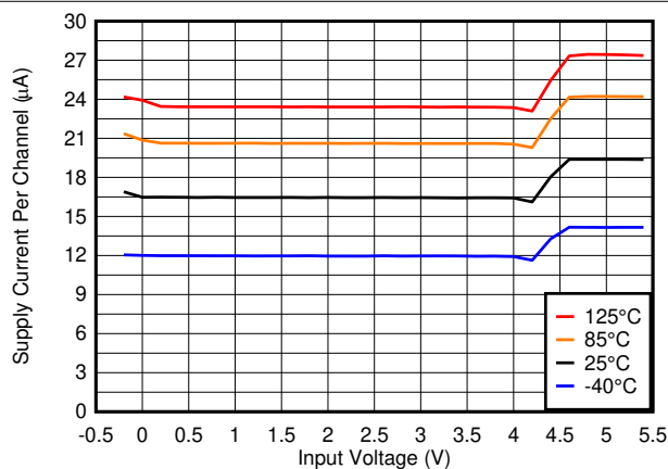
图 6-5. Supply Current vs. Input Voltage, 5V
