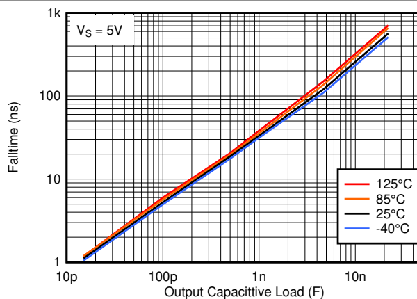
图 6-16. Falltime vs. Capacitive Load
