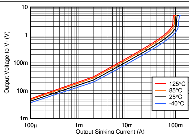
图 6-11. Output Sinking Current vs. Output Voltage, 5V
