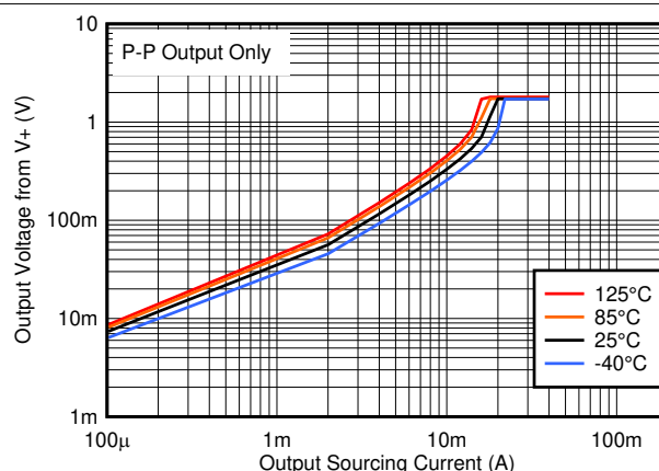
图 6-8. Output Sourcing Current vs. Output Voltage, 1.8V
