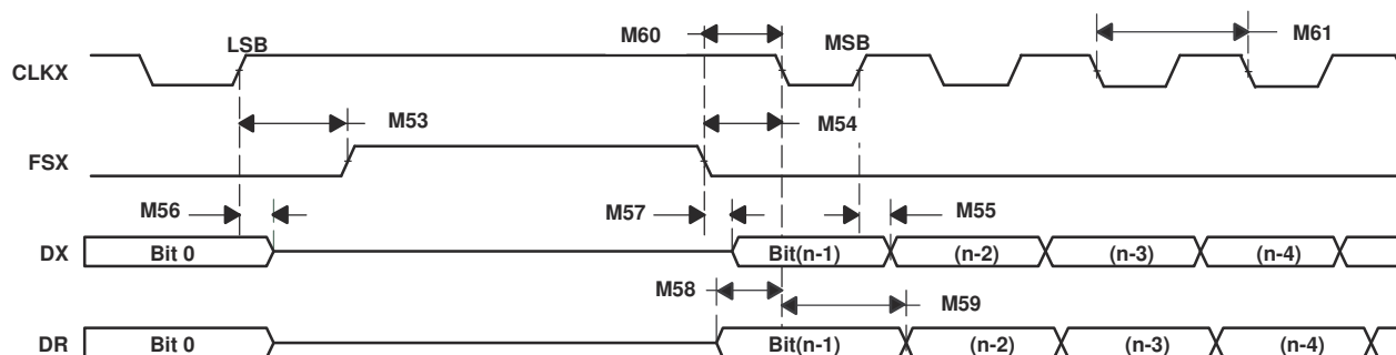
图 7-25. McBSP Timing as SPI Master or Slave: CLKSTP = 11b, CLKXP = 1
