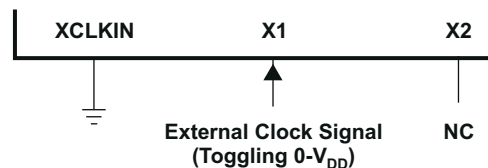
图 8-30. Using a 1.8-V External Oscillator
