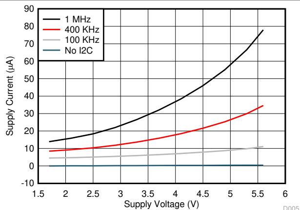
图 8-7. Supply Current vs. I²C Bus Clock and Supply Voltage in Shutdown Mode
