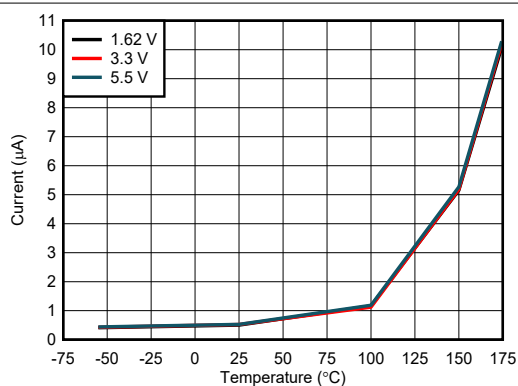
图 7-7. Standby Current vs Temperature
