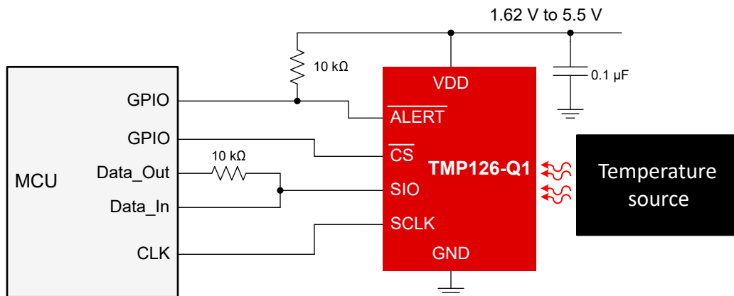
图 9-1. TMP126-Q1 Typical Connections
