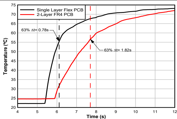
图 7-10. Stirred Liquid Response Time (DBV)
