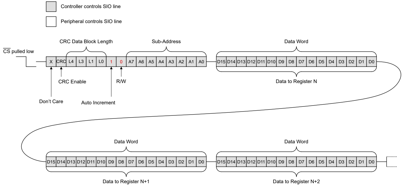
图 8-12. Burst Data Write to Multiple Registers
