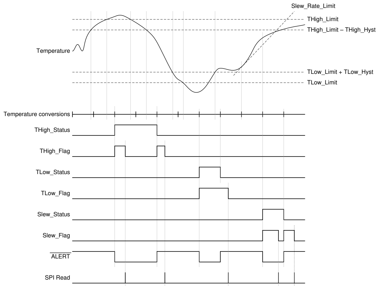
图 8-8. Comparator Mode Timing Diagram
