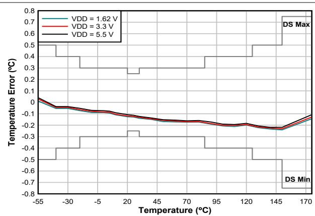
图 7-2. Average Temperature Accuracy (DCK)
