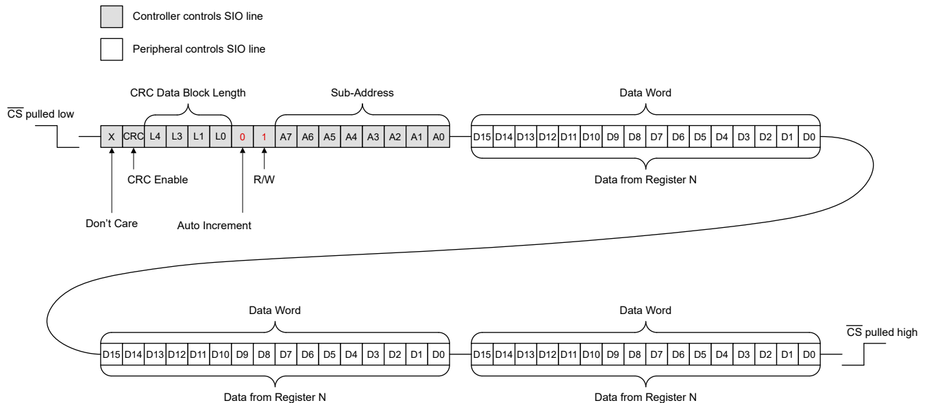
图 8-13. Repeated Data Read from a Single Register
