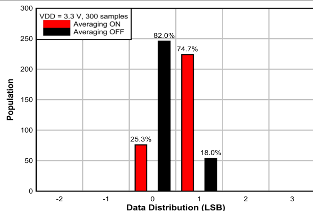
图 7-5. Temperature Measurement Noise Distribution at 175°C
