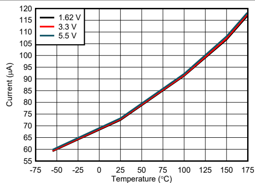
图 7-6. Active Conversion Current vs Temperature
