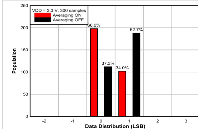
图 7-3. Temperature Measurement Noise Distribution at 25°C
