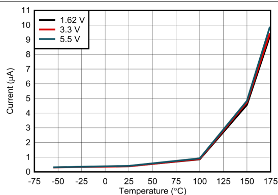
图 7-8. Shutdown Current vs Temperature
