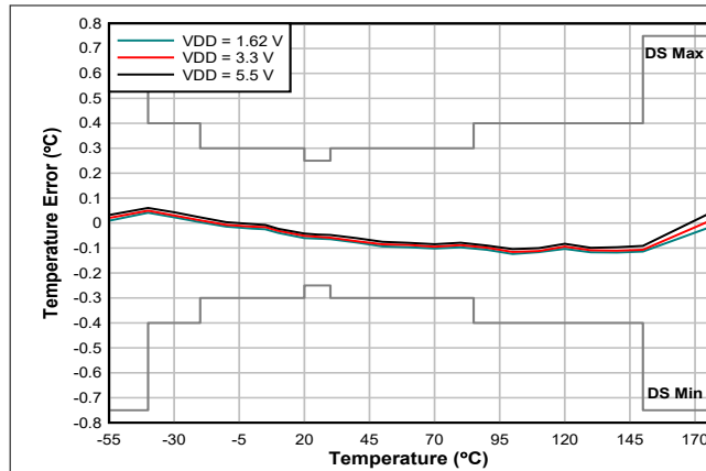
图 7-1. Average Temperature Accuracy (DBV)
