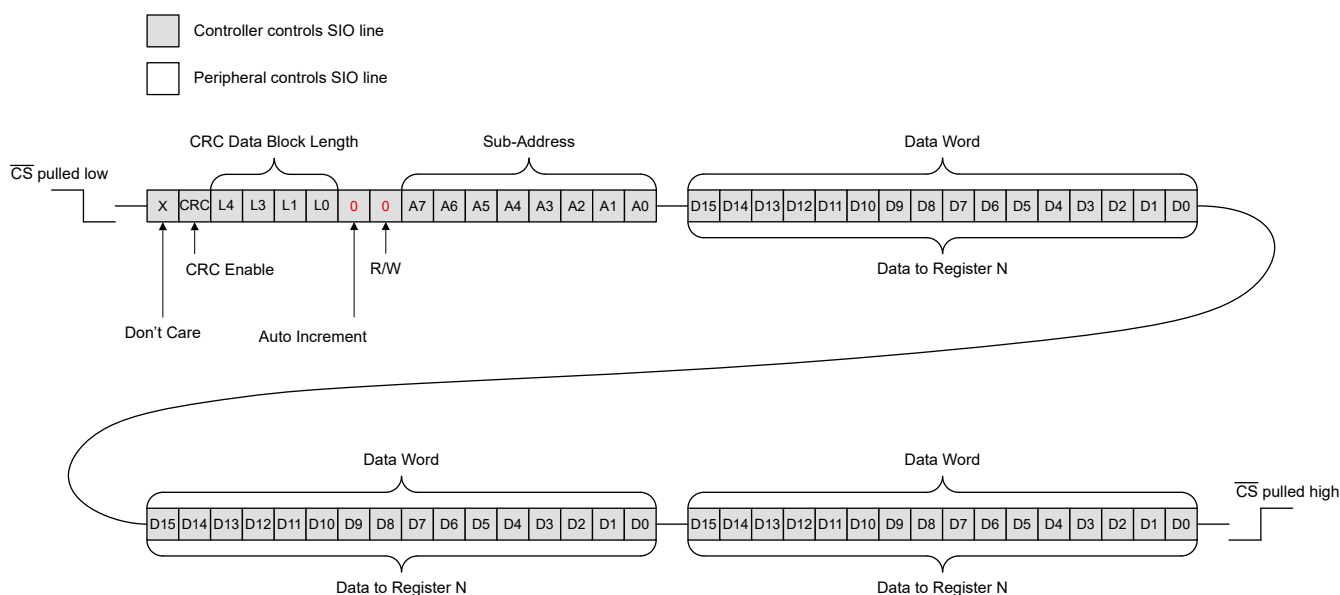
图 8-11. Repeated Data Write to a Single Register
