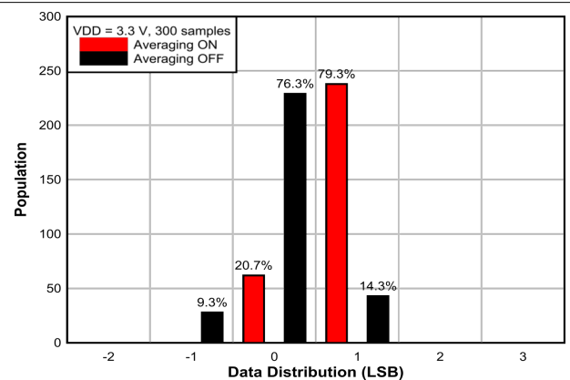
图 7-4. Temperature Measurement Noise Distribution at -55°C
