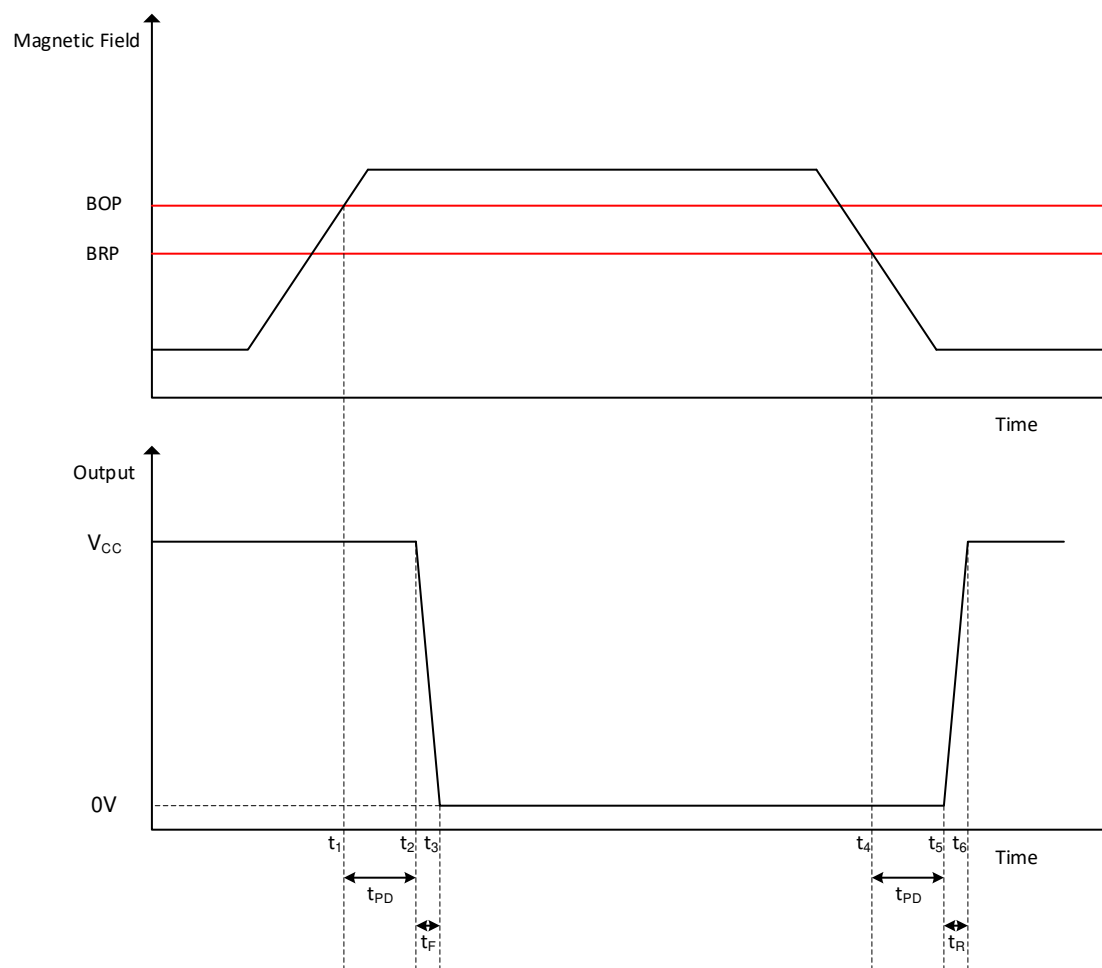
图 8-20. Propagation Delay
